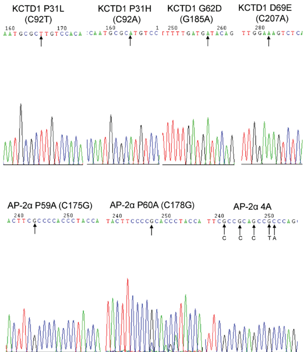
Figure S1. KCTD1 and AP-2 \alpha mutant sequences. KCTD1 and AP-2 \alpha sequences in recombinant plasmids were confirmed by Sanger sequencing analysis. KCTD1, potassium-channel tetramerization-domain-containing 1.
