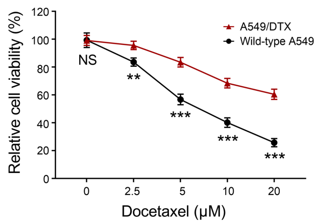
Figure S1. Docetaxel resistance in A549/DTX cells. ** P < 0.01 and *** P < 0.001 . NS, not significant.
