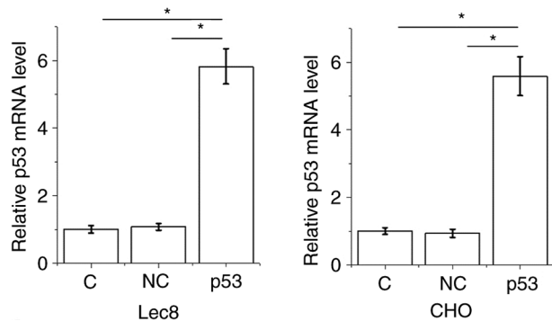
Figure S1. Confirmation of p53 overexpression in Lec8 and CHO cells after transient transfections using reverse transcription-quantitative PCR. *P<0.05. C, untransfected cells; NC, negative control (empty pcDNA3 vector).
