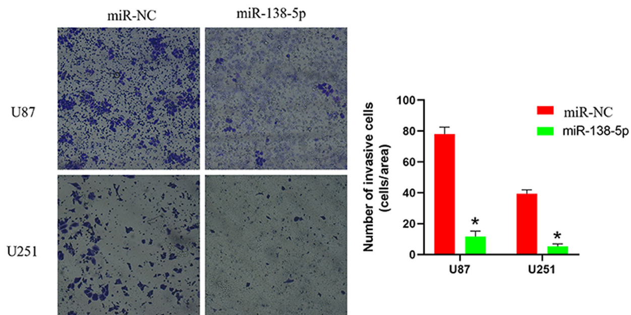
Figure S1. Invasive abilities of U87 and U251 cell lines transfected with the miR-138-5p mimic or miR-NC were analyzed using a Transwell assay. Magnification, x4. * P < 0.05 vs. miR-NC. An unpaired Student's t-test was used to analyze the data. miR, microRNA; NC, negative control.
