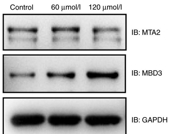
Figure S1. Detection of protein levels of MTA2 by immunoblotting following propofol treatment. A549 cells were treated with propofol for 72 h and protein expression levels of MTA2 and MBD3 were detected by immunoblotting. MTA2, metastasis-associated 1 family member 2; MBD3, methyl-CpG binding domain protein 3; IB, immunoblot.
