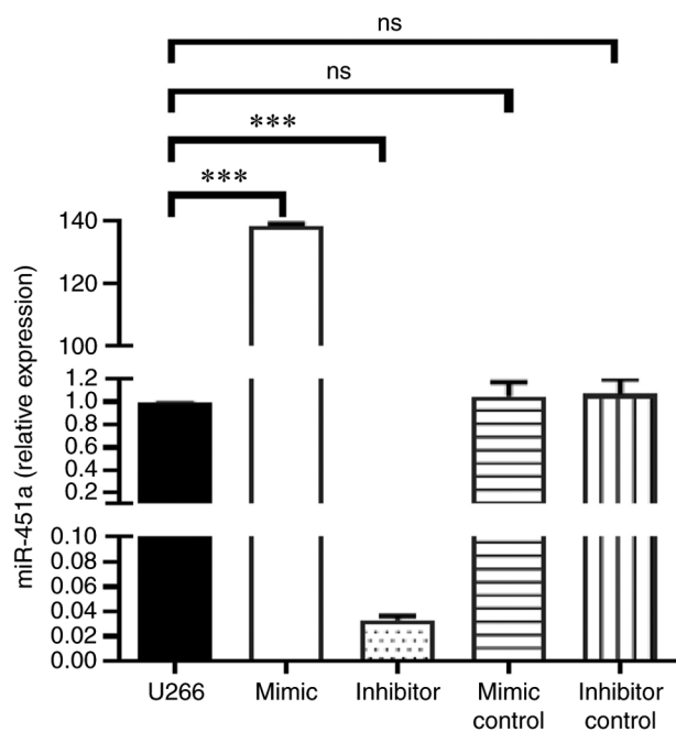
Figure S1. miR-451a expression levels following transfection. The levels of miR-451a increased or decreased in U266 cells transfected with miR-451a mimic or miR-451a inhibitor, respectively. Transfection with miR-451a mimic/inhibitor negative control did not significantly alter miR-451a levels. *** P < 0.0001 . miR, microRNA.
