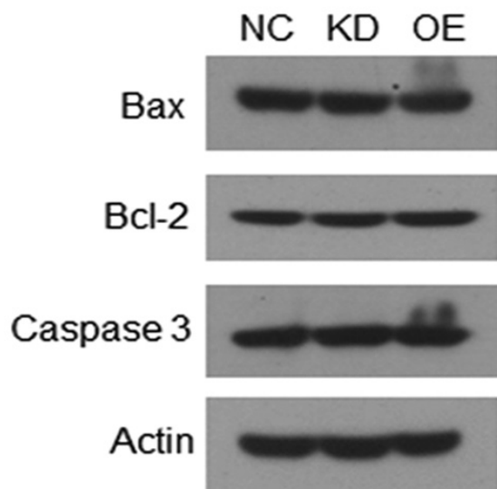
Figure S1. circFOXO3 shows no effects on the apoptotic pathway in the absence of radiation in cardiomyocytes. Protein expression levels of Bax, Bcl-2 and caspase-3 were evaluated by western blotting in AC16 cells with or without circFOXO3 KD or OE in the absence of radiation. circ, circular RNA; OE, overexpression; KD, knockdown; NC, negative control.
