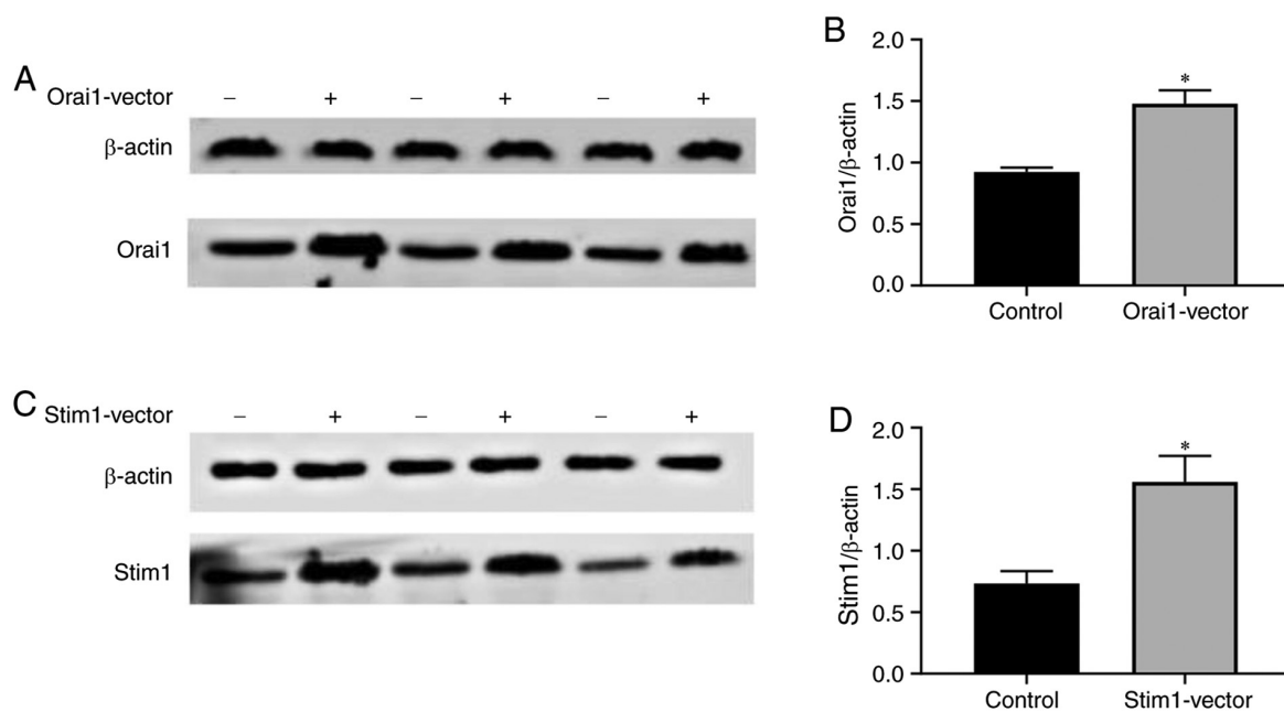
Figure S1. Confirmation of validity of STIM1 and Orai1 overexpression vector. (A) A representative image of western blot analysis performed for the analysis (B) of the expression of STIM1 in lung cancer A549 cells transfected with or without STIM1 overexpression vector. (C) A representative image of western blot performed for the analysis (B) of the expression of Orai1 in lung cancer A549 cells transfected with or without Orai1 overexpression vector. \beta -actin was used as loading control. Values are shown as the mean \pm standard deviation. n=3 . * P<0.05 vs. control group. STIM, stromal interaction molecule; Orai, calcium release-activated calcium channel protein.
