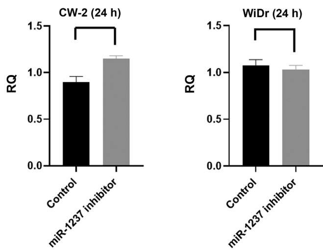
Figure S1. miR-1237 expression after miR-1237 inhibitor transfection was confirmed using real-time RT-PCR.
