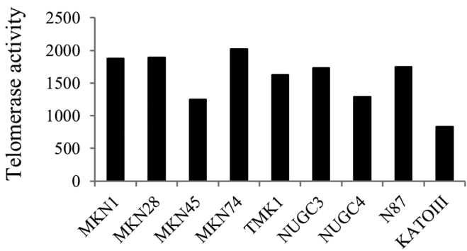
Figure S1. Telomerase activity in human gastric cancer cell lines.
