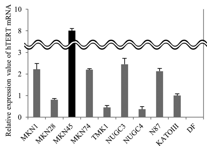
Figure S2. mRNA expression levels of hTERT in human gastric cancer cell lines. DF, dermal fibroblast; hTERT, human telomerase reverse transcriptase.
