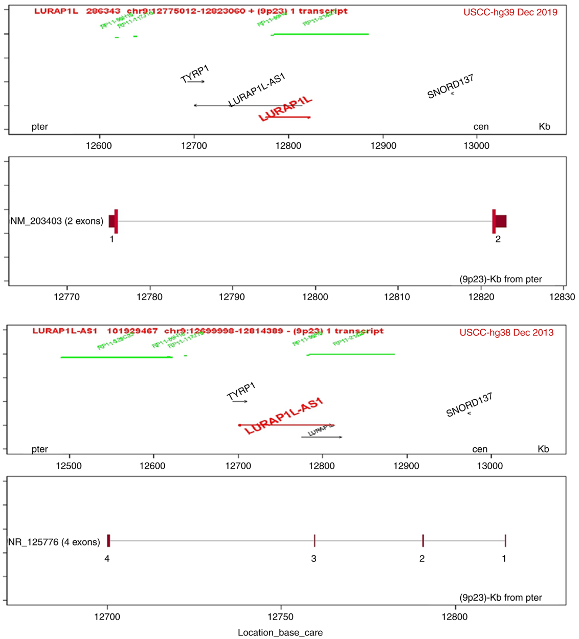
Figure S1. Prediction of correlation between LURAPIL-AS1 and LURAPIL. LURAPIL, leucine-rich adaptor protein 1-like; LURAPIL-AS1, LURAPIL antisense RNA 1.
