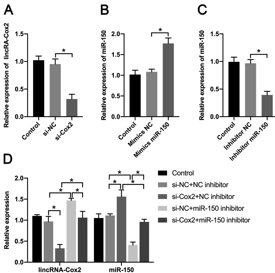
Figure S1. Efficiency of transfection. Efficiency of (A) si-Cox2, (B) mimics miR-150, (C) inhibitor miR-150, (D) si-Cox2 and inhibitor miR-150 in chondrocytes when co-transfected with si-Cox2 and miR-150 inhibitors. *P<0.05. linc, long intergenic non-coding; si, small interfering; NC, negative control; miR, microRNA.
