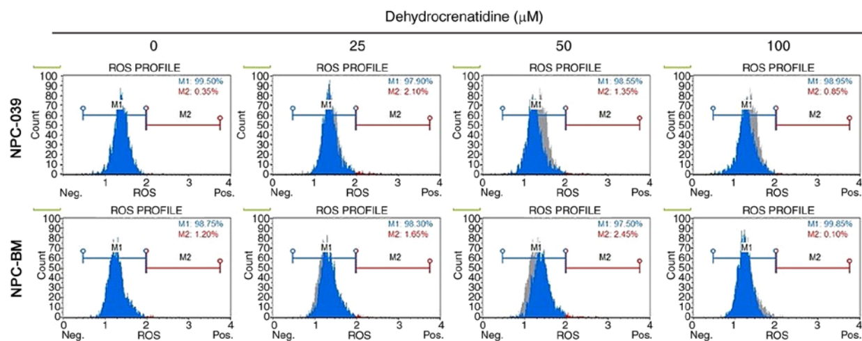
Figure S1. DC treatment does not increase ROS production in NPC cell lines NPC-039 and NPC-BM. (A) Reactive oxygen species (ROS) was analyzed after treatment with DC (0, 25, 50, and 100 \mu M) by using the Muse Cell Analyzer. NPC, nasopharyngeal carcinoma; DC, dehydrocrenatidine.
