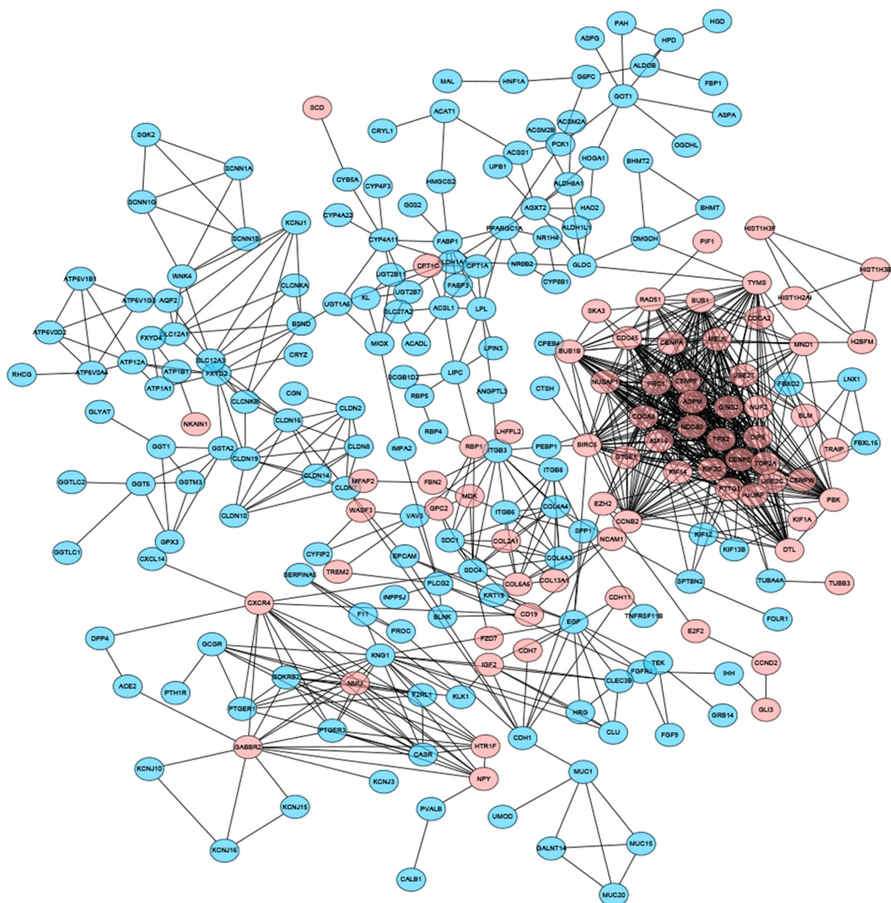
Figure S1. Protein-protein interaction network of common differentially expressed genes. Nodes represent proteins and lines represent interactions. Red nodes, upregulated genes; blue nodes, downregulated genes.
