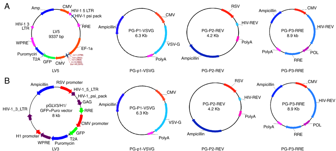
Figure S1. Lentiviral packaging systems. (A) Four-plasmid system for LV5 lentivirus. (B) Four-plasmid system for LV3 lentivirus.
