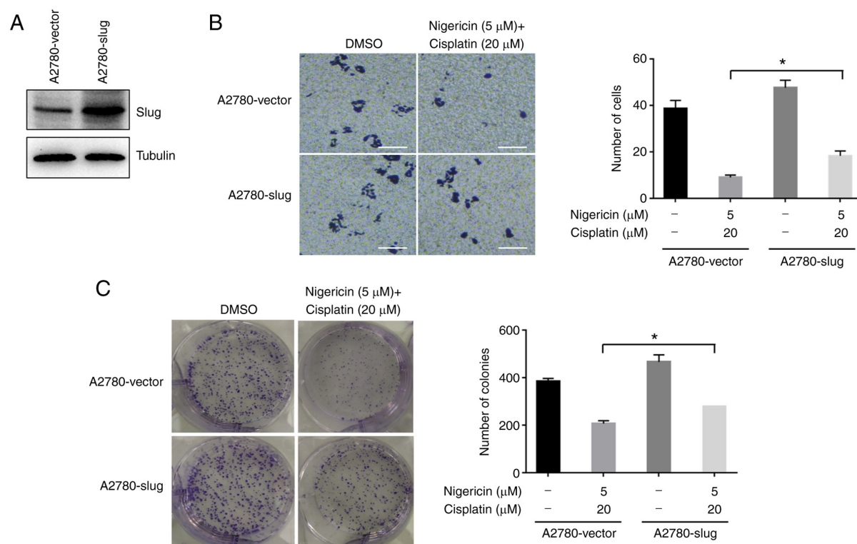
Figure S1. Overexpression of slug in A2780 cells rescues the phenotype induced by treatment with nigericin combined with cisplatin. (A) Slug expression was determined by western blotting. Tubulin was used as a control. Overexpression of slug rescued the inhibitory effect of nigericin and cisplatin on (B) migration and (C) colony formation. Scale bar, 50 \mu m. *P<0.01 vs. vector.
