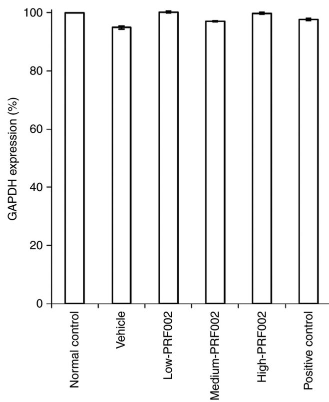
Figure S1. mRNA expression of GAPDH in cells isolated from the gastric wall and gastric mucosa. The groups were the normal control, vehicle, low-PRF002, medium-PRF002, high-PRF002 and positive control.
