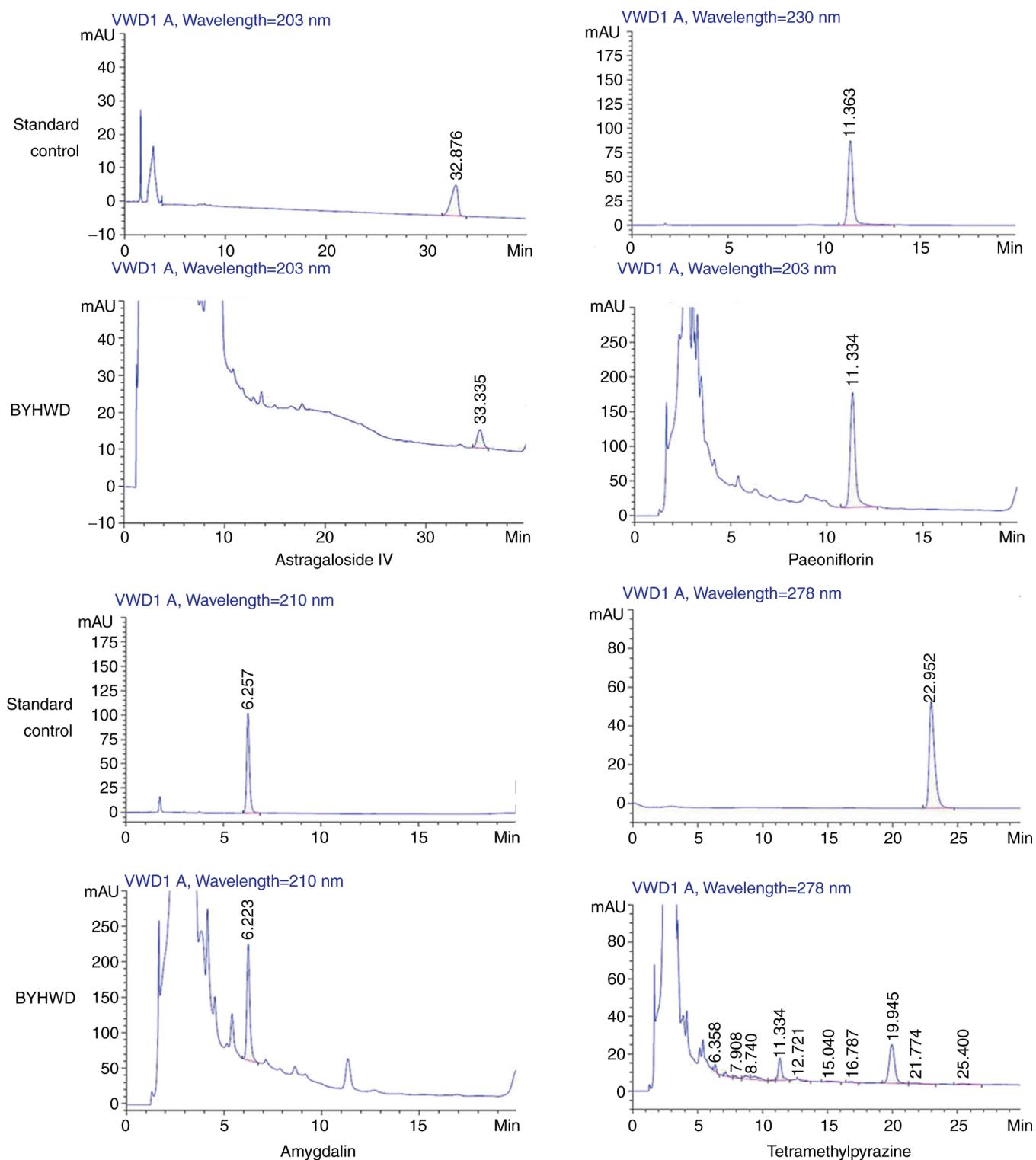
Figure S1. Representative HPLC chromatograms of active BHD components and standard controls. BHD contains astragaloside IV, paeoniflorin and amygdalin, but not tetramethylpyrazine; BHD, Buyang Huanwu Decoction.
