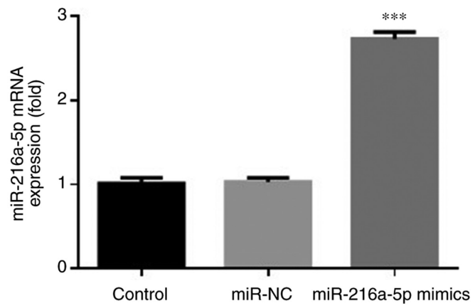
Figure S2. miR-216a-5p expression in different cell groups. Cells were transfected with control, miR-NC or miR-216a-5p mimics. ***P<0.001 vs. control. miR, microRNA; NC, negative control.
