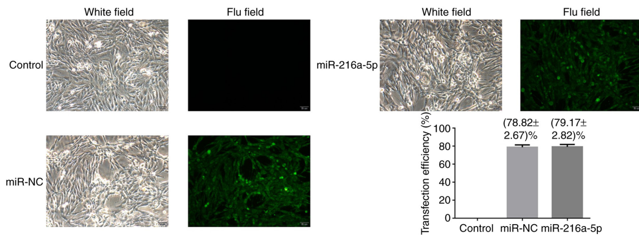
Figure S1. Transfection efficiency. Cells were transfected with control, miR-NC or miR-216a-5p mimics. miR, microRNA; NC, negative control.
