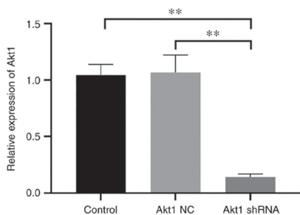
Figure S1. Reverse transcription-quantitative PCR analysis of Akt1 expression in C4-2 cells transfected with Akt1shRNA, AktNC or Control. Data are expressed as the mean \pm SD (n=3); each bar represents the mean of three independent experiments carried out in triplicate. **P<0.01. shRNA, short hairpin RNA; NC, negative control.
