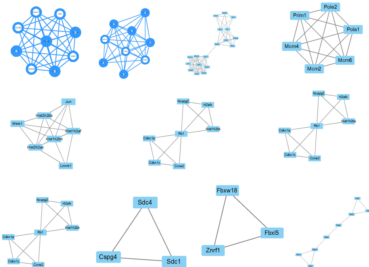
Figure S1. MCODE model of the differentially expressed genes.
