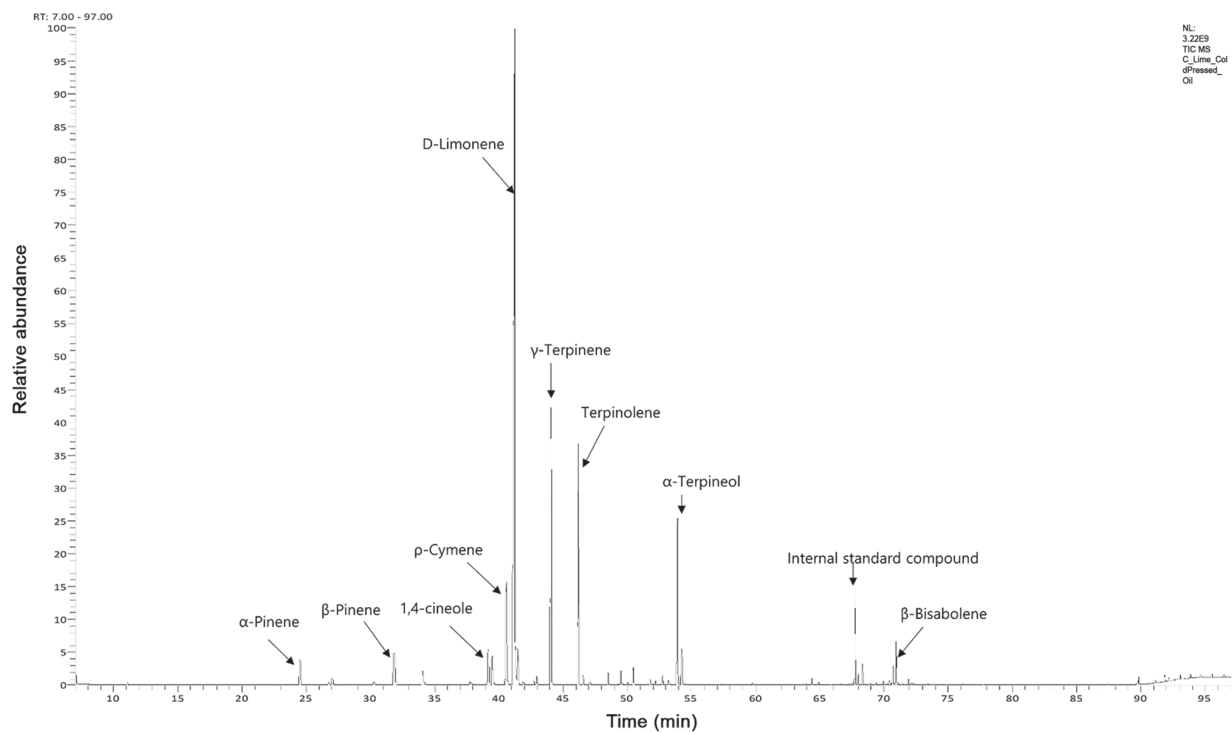
Figure S1. Gas chromatography-mass spectrometry traces of lime cold-pressed oil.
