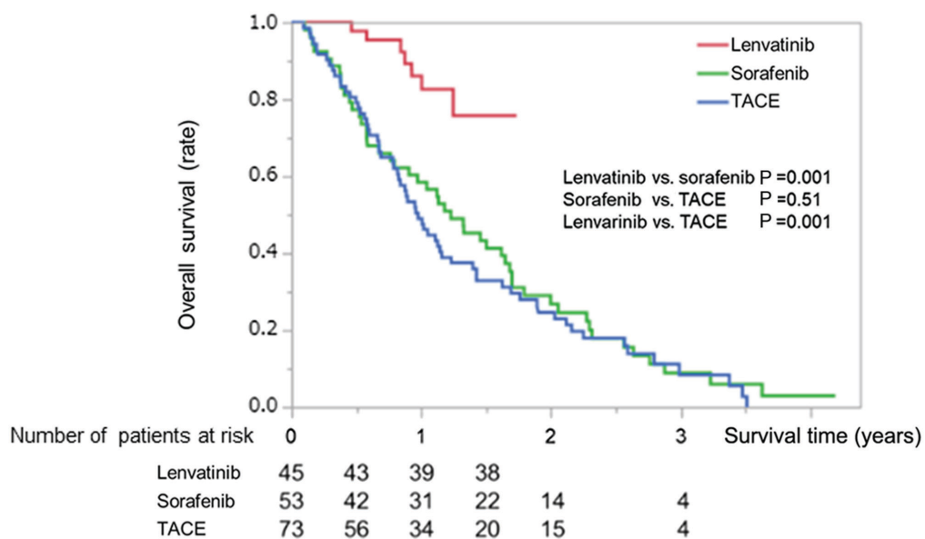
Figure S1. Kaplan-Meier curves for overall survival in the lenvatinib, sorafenib and TACE groups. TACE, transarterial chemoembolization.
