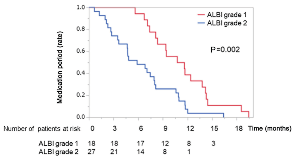
Figure S2. Kaplan-Meier curves for the medication period with lenvatinib in the ALBI grade 1 and 2 groups. ALBI, albumin-bilirubin.
