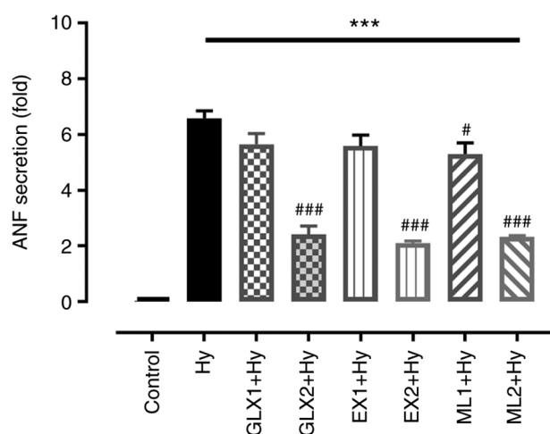
Figure S1. Preliminary tests of inhibitors on the regulation of hypoxia-induced ANP secretion in isolated beating rat atria (n=3). GLX1, IC 50 dose of GLX351322 (5 \mu M); GLX2, effective dose of GLX351322 (35 \mu M); EX1, IC 50 dose of EX3527 (123 nM); EX2, effective dose of EX527 (0.25 \mu M); ML1, IC 50 dose of ML385 (1.9 \mu M); ML2, effective dose of ML385 (10 \mu M). ***P<0.001 vs. control; #P<0.05, ###P<0.001 vs. Hy. Hy, hypoxia.
