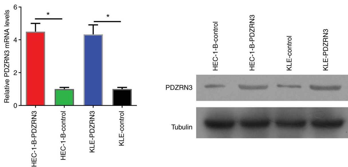
Figure S1. Expression levels of PDZRN3 in endometrial cancer cells. PDZRN3 expression was identified by reverse transcription quantitative PCR and western blotting. *P<0.05. PDZRN3, PDZ Domain Containing Ring Finger 3.
