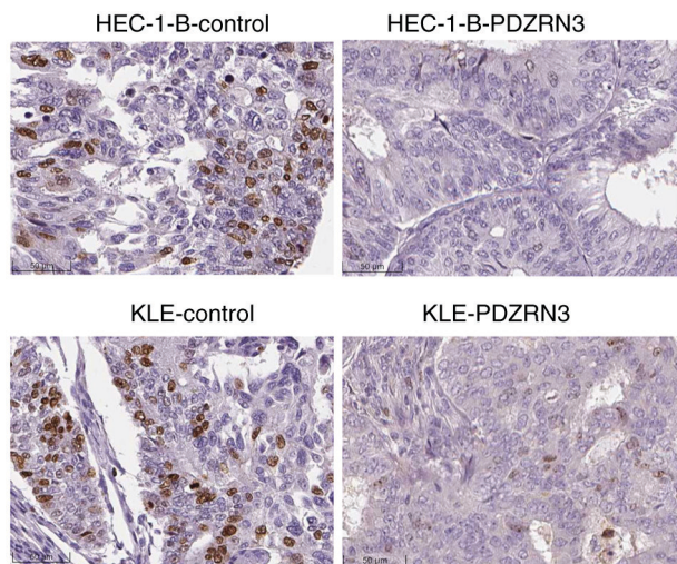
Figure S2. Expression levels of Ki-67 in subcutaneous tumor tissue in vivo . Ki-67 staining showed that ki-67 expression was low in PDZRN3-overexpressing groups. Magnification, x400. PDZRN3, PDZ Domain Containing Ring Finger 3.
