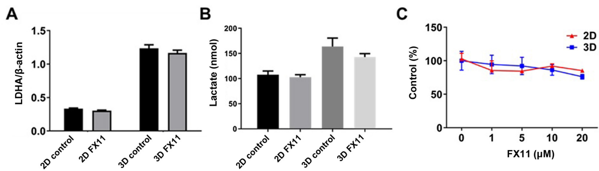
Figure S1. (A) LDHA expression level changes upon FX11 addition (B) changes in lactate secretion upon addition of FX11 in 2D and 3D SW480 (C) 2D and 3D SW480 viability changes upon addition of FX11.
