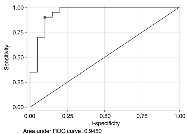
Figure S2. ROC curve for angiopoietin-like 4. The optimal cut-point was indicated by a single mark on the ROC curve. ROC, receiver operating characteristic.
