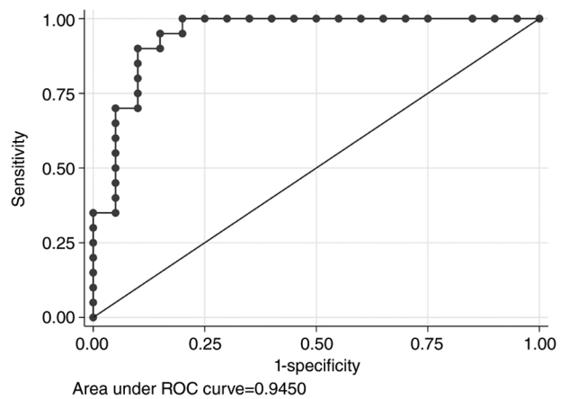
Figure S1. ROC curve for angiotensin-like 4 level to discriminate patients with lung metastasis from patients with no metastasis. The area under the ROC curve was 0.9450. ROC, receiver operating characteristic.
