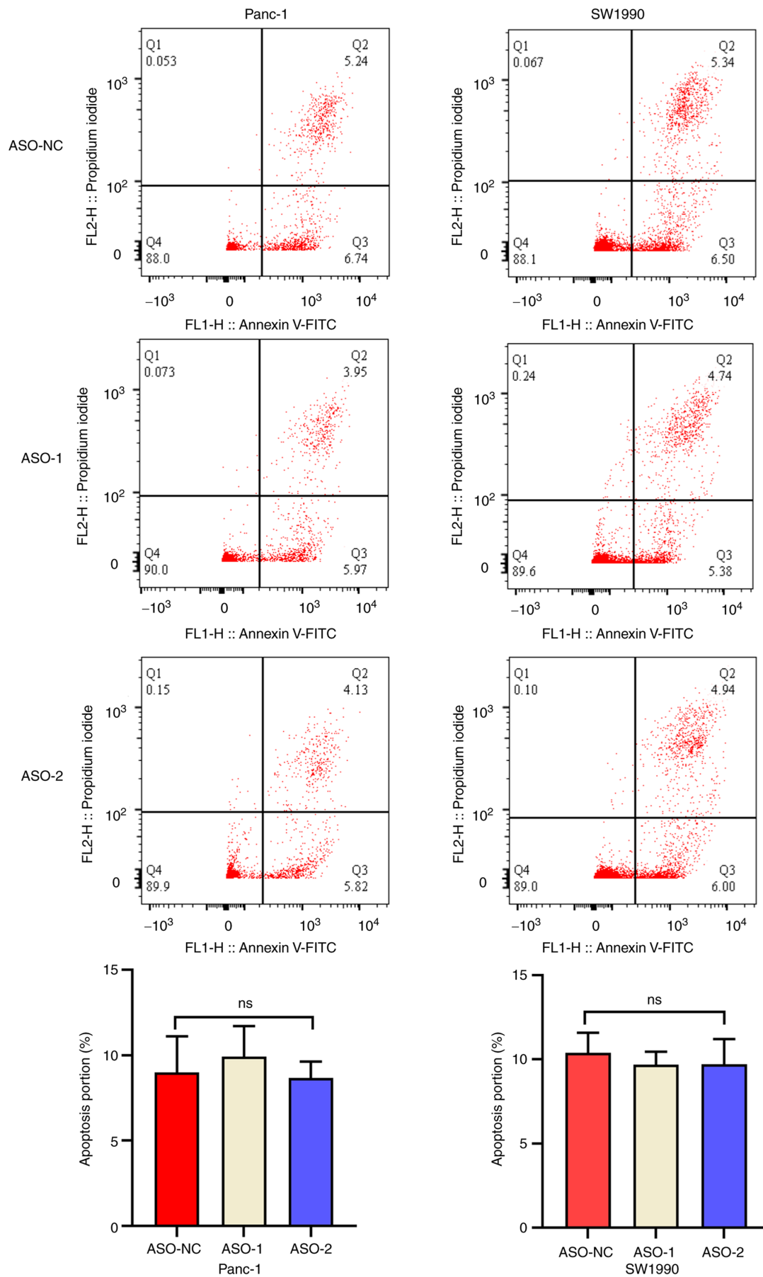
Figure S1. Flow cytometry results demonstrating that linc01614 knockdown had no significant effect on the apoptosis of Panc-1 and SW1990 cells.
