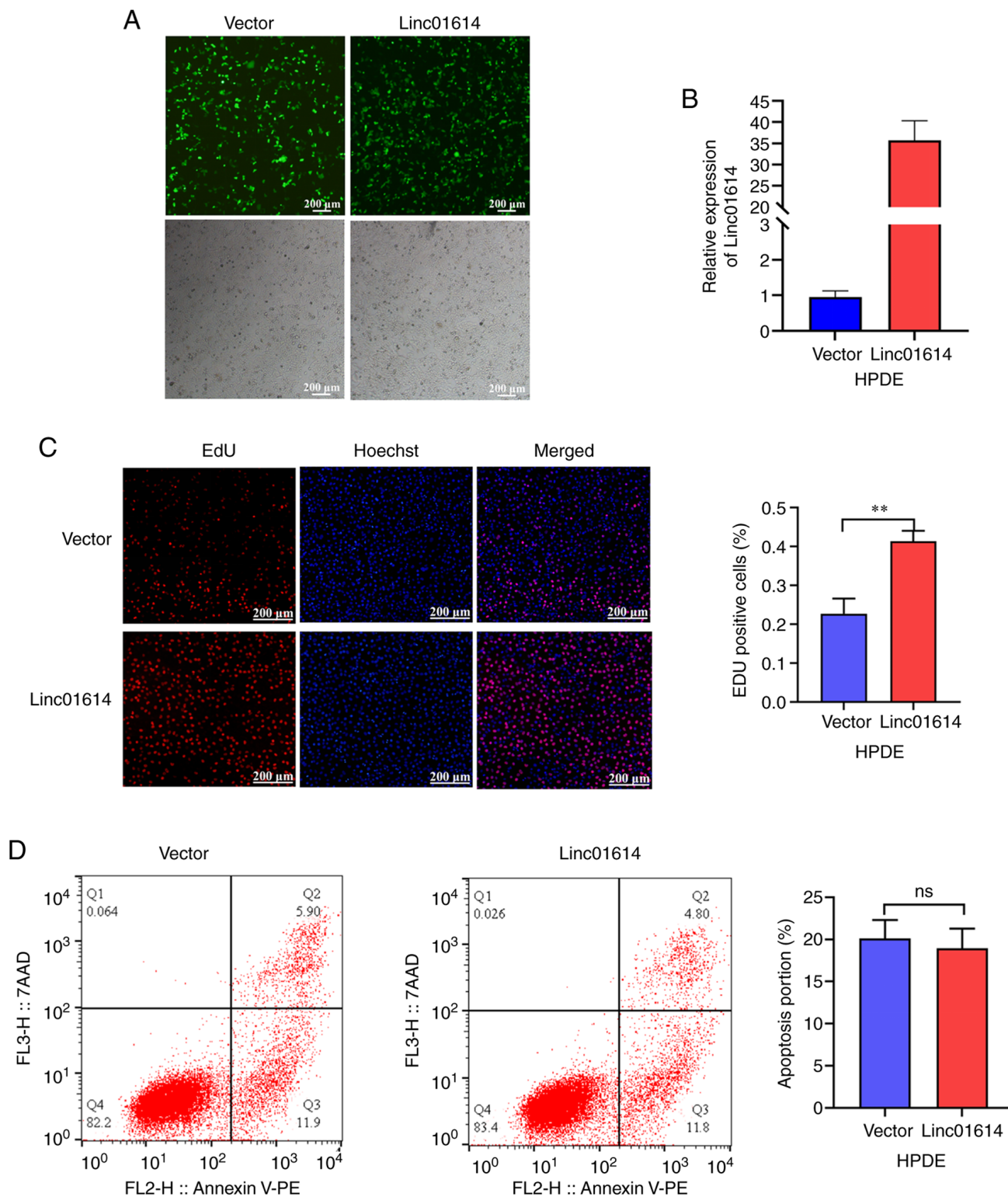
Figure S2. Effects of linc0164 upregulation on HPDE cells. (A) Representative images of HPDE cells transfected with linc01614 plasmid and negative control (vector). Magnification, x100. (B) reverse transcription-quantitative polymerase chain reaction for the evaluation of linc01614 transfection efficacy in HPDE cells. (C) EdU assay for the evaluation of the increase in HPDE cell proliferation upon the upregulation of linc01614. Magnification, x200. (D) Flow cytometry demonstrated no significant effect on the apoptosis in HPDE cells, following linc01614 overexpression. Data are presented as the mean \pm SD. ** P < 0.01 vs. the negative control (ns, not significant).
