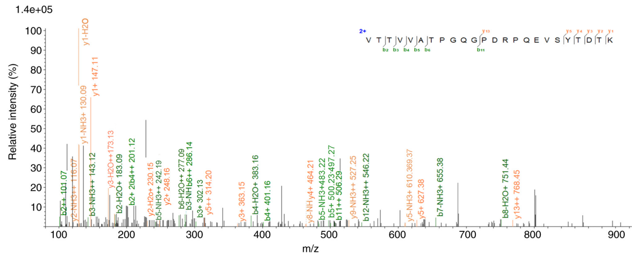
Figure S3. Mass spectrometry illustrating the GSK-3β peptides.
