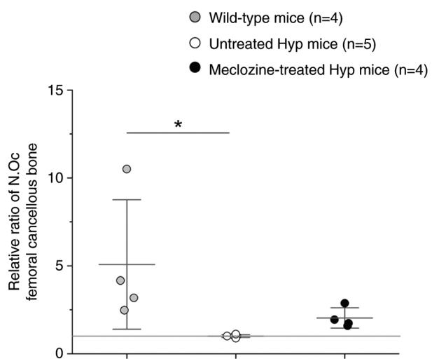
Figure S1. N.Oc. Dots indicate the relative N.Oc, and bars indicate the mean \pm SD. Statistical significance was analyzed by one-way ANOVA with post-hoc Tukey's honest significance test. * P < 0.05 . Hyp mice, X-linked hypophosphatemic mice; N.Oc, number of osteoclasts.
