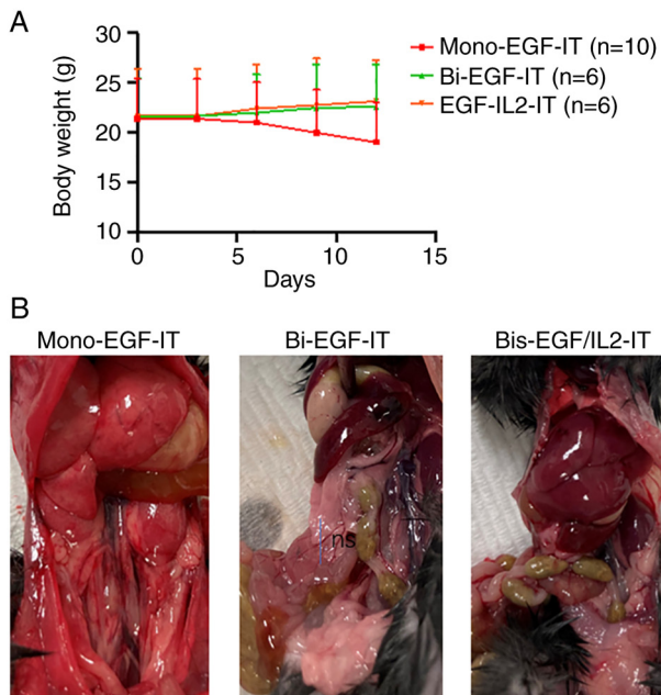
Figure S1. Necropsy results for C57BL/6 mice treated with mono-EGF-IT, bi-EGF-IT, or bis-EGF/IL2-IT in the absence of tumor inoculation. C57BL/6 mice were treated with mono-EGF-IT (n=10), bi-EGF-IT (n=6), or bis-EGF/IL2-IT (n=6). Mice were euthanized on day 13 after the first injection of the fusion toxins. (A) Body weight of mice was recorded and plotted along the observation period. (B) Gross changes in the abdominal cavity are shown. IT, immunotoxin.
