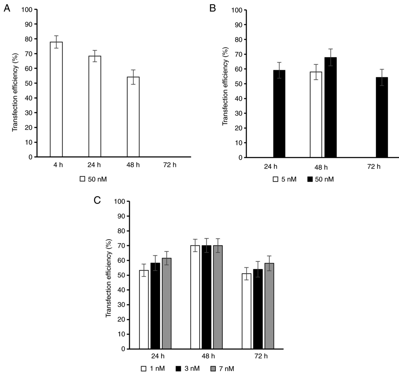
Figure S1. Transfection efficiency. (A) Transfection with nucleofection (50 nM hsa-miR-302b-3p) after 4, 24, 48 and 72 h. (B) Transfection with Viromer® Blue (5 and 50 nM hsa-miR-302b-3p) after 24, 48 and 72 h. (C) Transfection with INTERFERin® (1, 3 and 7 nM hsa-miR-302b-3p) after 24, 48 and 72 h. Data are presented as the mean \pm SD.
