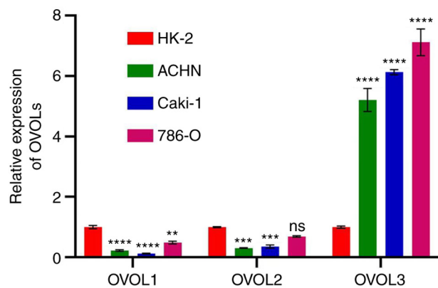
Figure S1. The expression of distinct OVOL1, OVOL2 and OVOL3 in healthy kidney and clear cell renal cell carcinoma cell lines. OVOL1 , OVOL2 , and OVOL3 mRNA levels in healthy kidney and clear cell renal cell carcinoma cell lines were determined using. **P<0.01, ***P<0.001, ****P<0.0001. ns, not significant.
