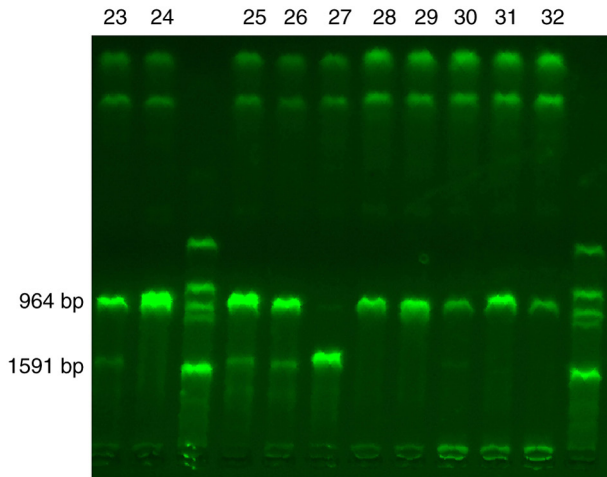
Figure S1. DNA electrophoresis strip image. The wild-type was 1,591 bp and the adropin knockout homozygote was 964 bp. The lane numbers correspond to the ear tag numbers assigned to each mouse.
