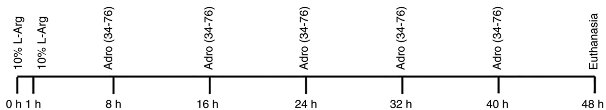
Figure S2. Information of the administration route and schedule of the animal experiment. L-Arg, L-arginine; Adro, adropin.
