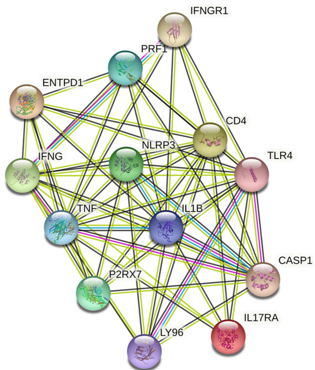
Figure S1. Protein-protein interaction of differentially expressed immunogenic cell death-related genes in pancreatic cancer.
