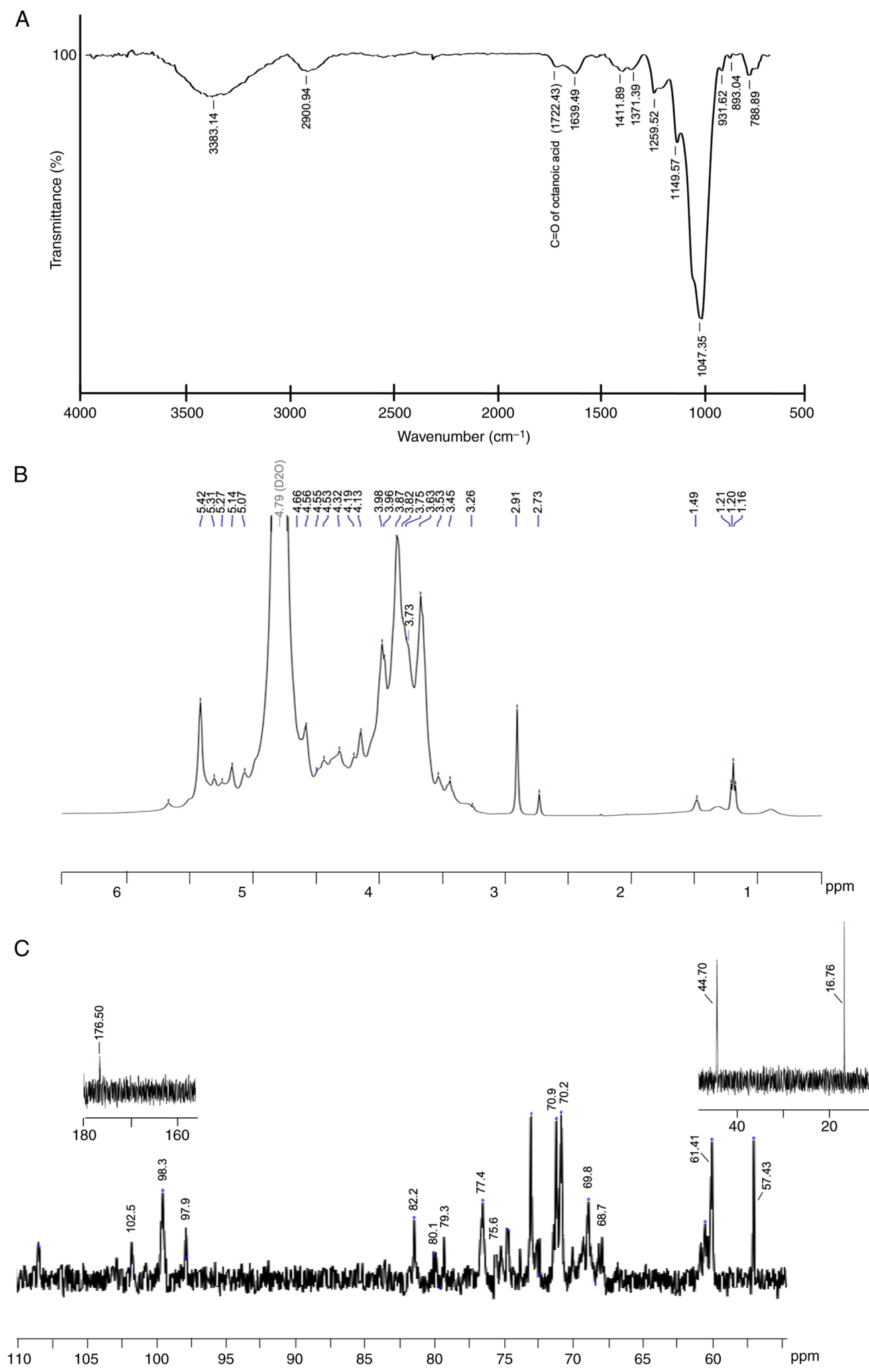
Figure S1. (A) Fourier-transform infrared spectral analysis of Oct-LMSG, (B) ^1\text{H} -NMR spectral analysis of Oct-LMSG and (C) ^{13}\text{C} -NMR spectral analysis of Oct-LMSG. Oct-LMSG, low molecular weight sulfated galactan added with octanoyl moiety.
