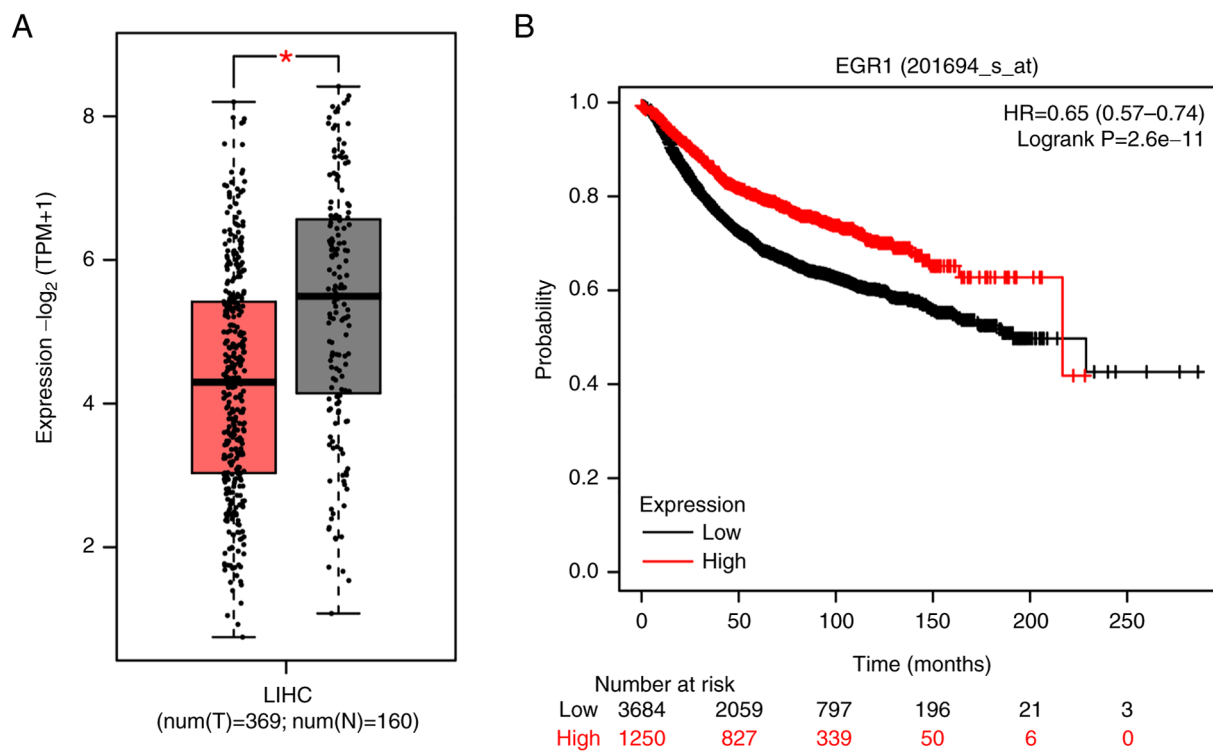
Figure S1. Expression level and prognostic result of EGR1 in patients with LIHC. (A) Box plot showing the expression level of EGR1 in patients with LIHC. *P<0.05. (B) Line plot showing the prognostic result by dividing patients with LIHC into two groups according to EGR1 expression levels. LIHC, liver hepatocellular carcinoma; HR, hazard ratio.
