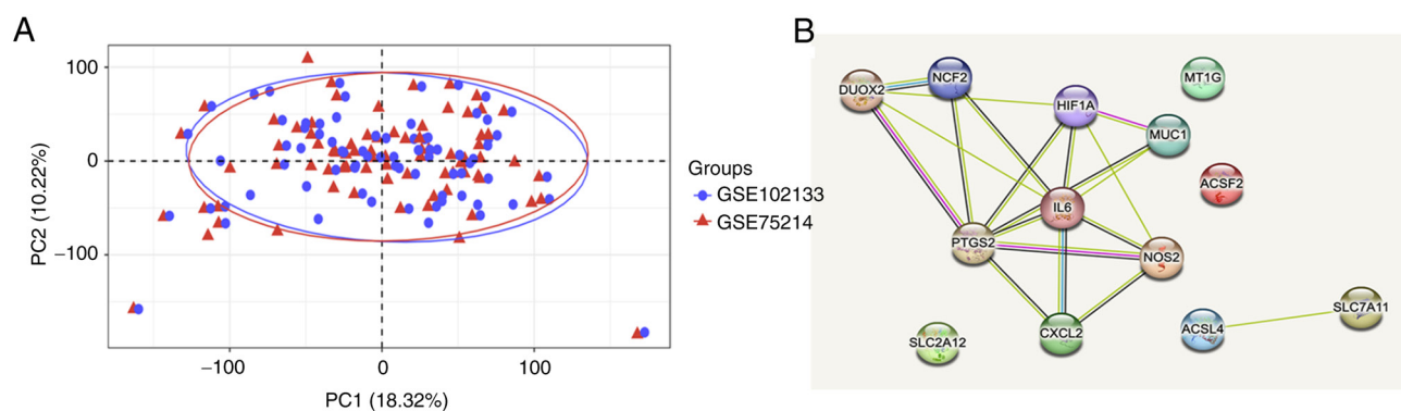
Figure S1. PCA image and PPI network based on STRING. (A) PCA result. (B) PPI network between the 13 ferroptosis-related genes based on STRING. PCA, principal component analysis; PPI, protein-protein interaction; STRING, Search Tool for the Retrieval of Interacting Genes.
