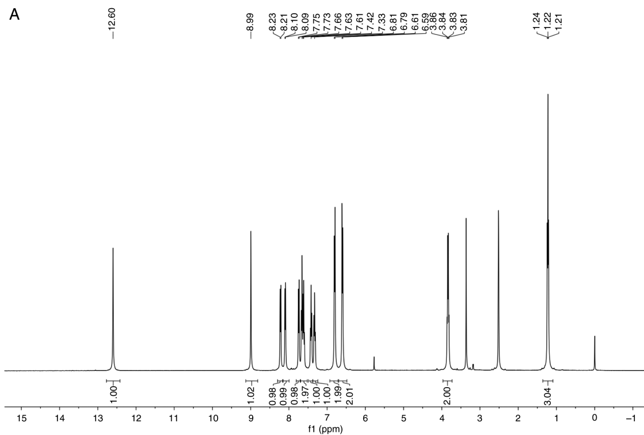
Figure S1. NMR spectroscopy of compound 225#. (A) ^1\text{H} -NMR spectrum of compound 225# and (B) ^{13}\text{C} -NMR spectrum of compound 225#. NMR, nuclear magnetic resonance.
