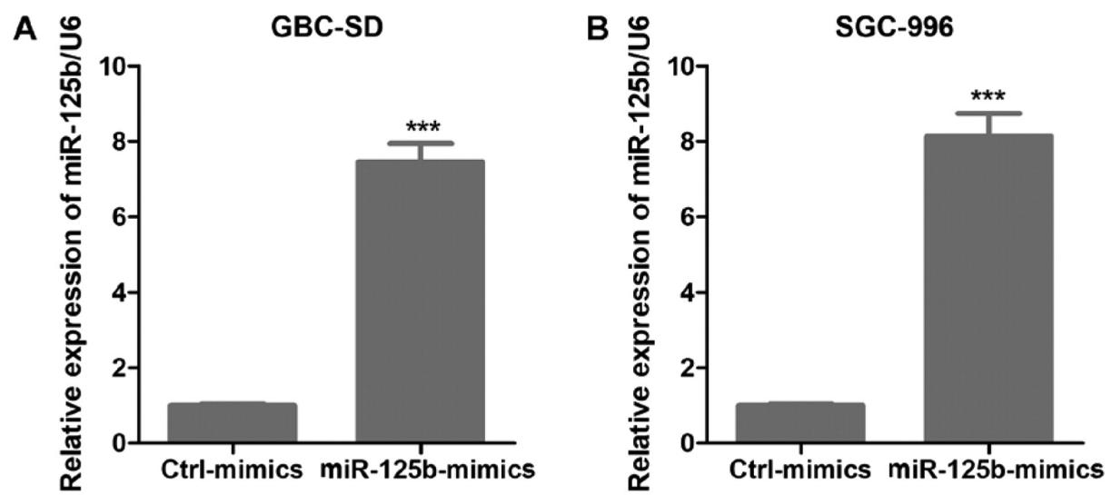
Figure S1. miR-125b overexpression in GBS-SD and SGC-996 cells. miR-125b expression levels in (A) GBC-SD and (B) SGC-996 cell transfected with Ctrl-mimics or miR-125b-mimics. U6 was used as the internal control. ***P<0.001.
