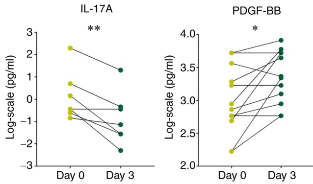
Figure S1. Intraindividual changes in urinary cytokines in patients with ccRCC before and after surgery. Individual dot plot shows the urinary cytokines whose levels changed significantly in the majority of patients with ccRCC after tumor removal. Day 0 corresponds to the preoperative urine of patients, while day 3 corresponds to the urine of patients collected on the 3rd day after removal of the tumor. * P \leq 0.05 and ** P \leq 0.01 (paired t-test). ccRCC, clear cell renal cell carcinoma; PDGF-BB, platelet-derived growth factor-BB.
