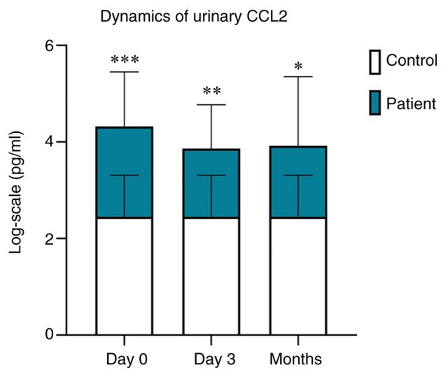
Figure S2. Urinary CCL2 levels in patients with ccRCC before and at different time intervals after surgery. The stacked bar chart shows the levels of CCL2 in urine samples collected from patients with ccRCC at different time intervals: Prior to surgery, on the 3rd day after surgery and on average 10 months after the tumor was removed compared with controls. * P \leq 0.05 , ** P \leq 0.01 and *** P \leq 0.001 for patients versus controls. ccRCC, clear cell renal cell carcinoma; CCL, chemokine (C-C motif) ligand.
