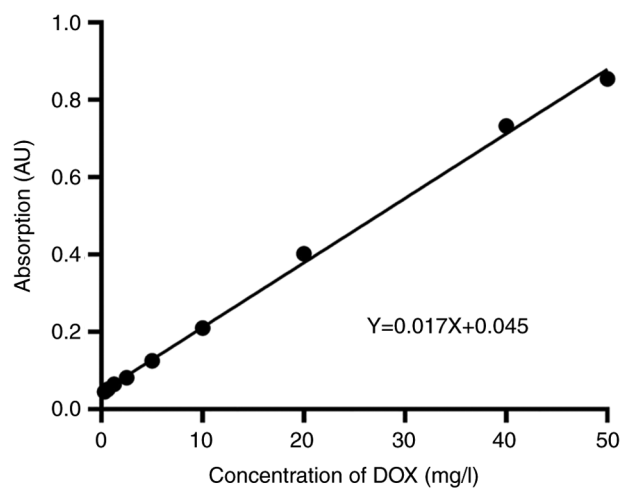
Figure S1. Ultraviolet standard curve of DOX in aqueous solution. The DOX concentrations used were 0.3125, 0.625, 1.25, 2.5, 5, 10, 20, 40 and 50 mg/l. DOX, doxorubicin.
