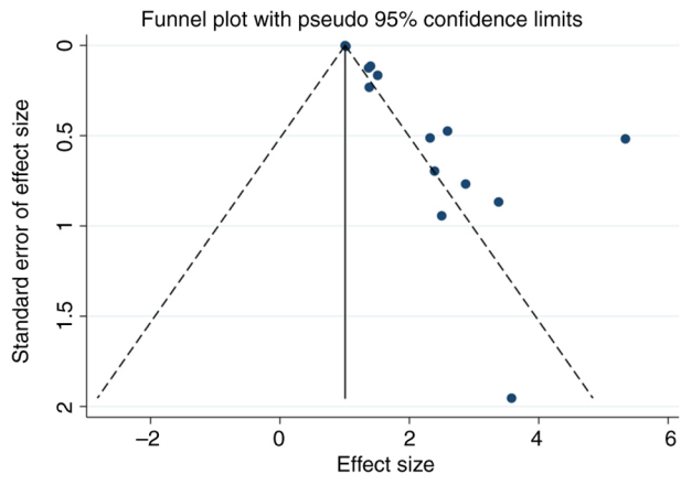
Figure S1.Funnel plot.
