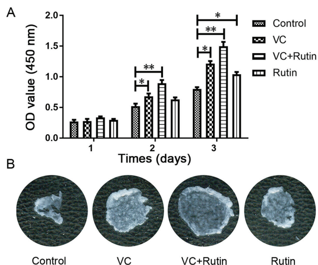
Figure S1. Combined treatment with VC and rutin promotes the formation of PDLSC sheets. PDLSCs were cultured in \alpha -minimum essential medium with or without VC (20 \mu g/ml) and rutin ( 1 \times 10^{-6} mol/l) for 3 days. (A) OD values of the control group, VC group, VC + rutin group and rutin group on day 3. (B) Representative images of cell sheets in culture dishes. * P < 0.05 , ** P < 0.01 . VC, vitamin C; PDLSC, periodontal ligament stem cell.
