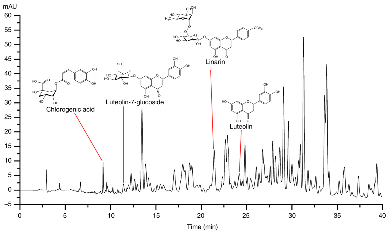
Figure S1. High-performance liquid chromatograph of the 75% methyl alcohol layers of the supercritical carbon dioxide fluid extraction of Chrysanthemum indicum Linnén. mAU, m absorbance unit.
