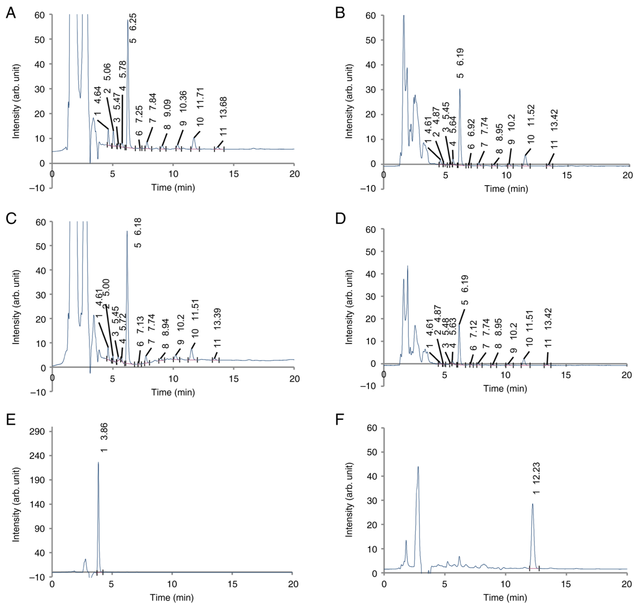
Figure S1. High performance liquid chromatography chromatograms of LH and LT. Chromatograms of LH were recorded at (A) 214 and (B) 280 nm. Chromatograms of LT were recorded at (C) 214 and (D) 280 nm. Chromatograms of (E) formononetin and (F) lespedezaflavanone H were recorded at 214 nm.
