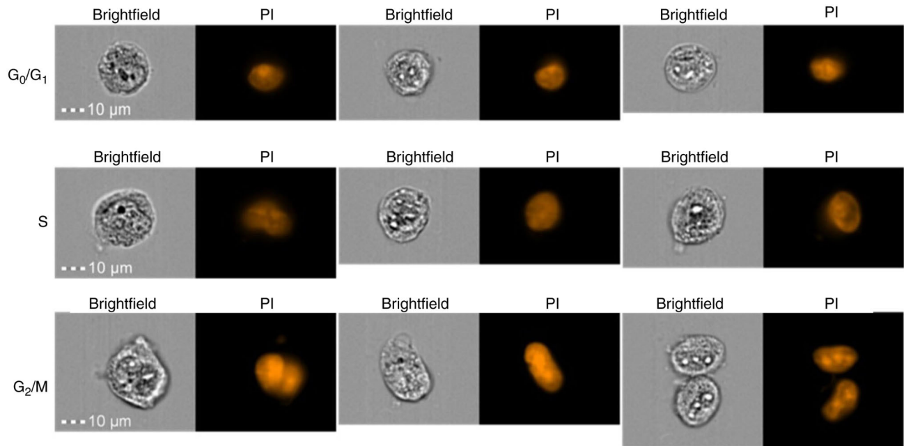
Figure S1. Cell cycle phases. Representative images of MDA-MB-231 triple-negative breast cancer cells in the G_0/G_1 , S and G_2/M phases of the cell cycle. The scale bar shown in the first image of each row can be applied to every image in that row. Three repeats are shown in each row.
