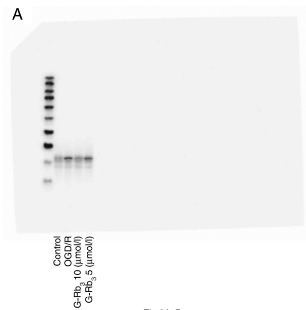
Fig.2A: Bax
