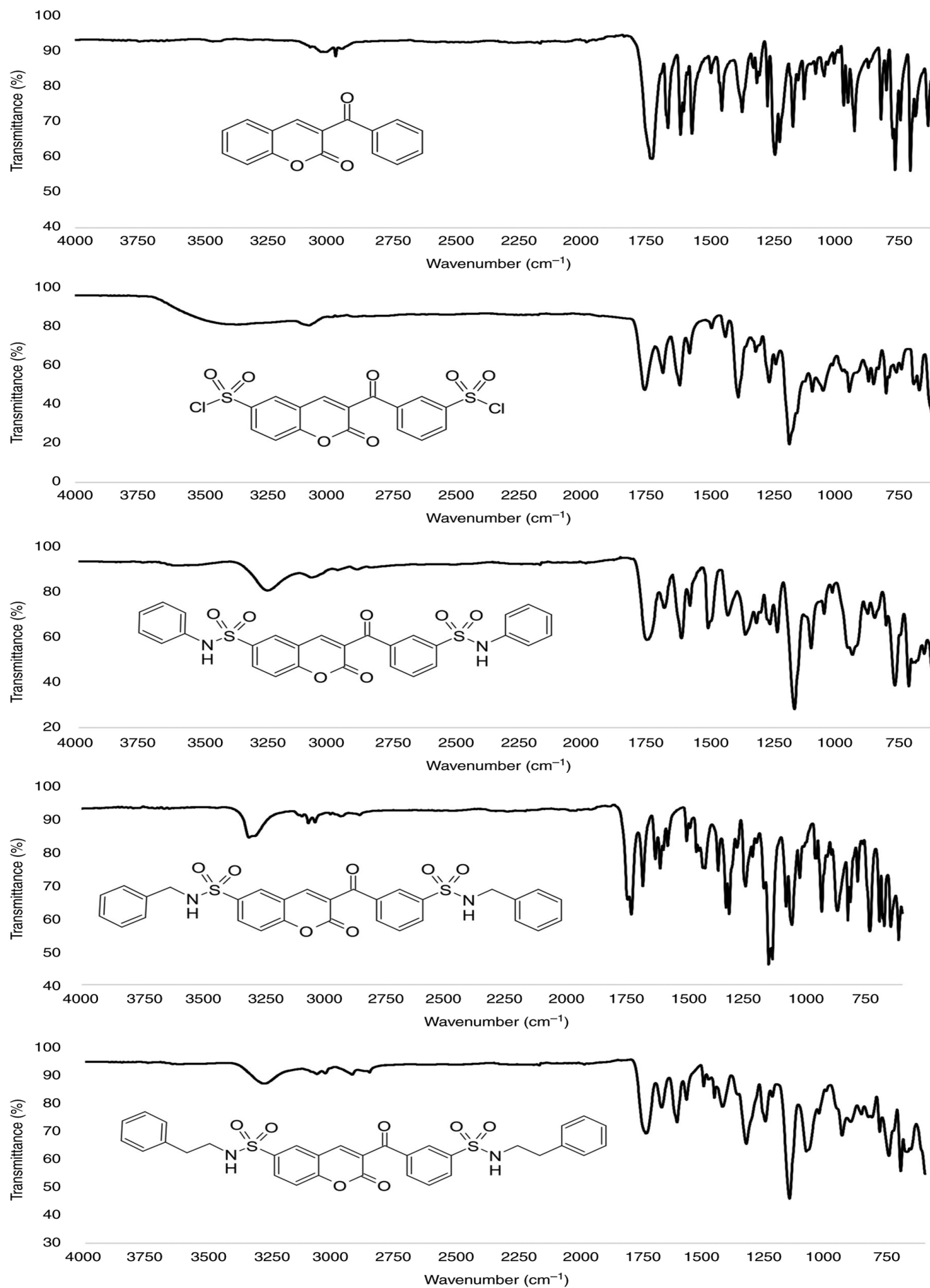
Figure S2. IR spectra ( \text{cm}^{-1} ) of compounds 6, 7, 8a, 8b and 8c.
