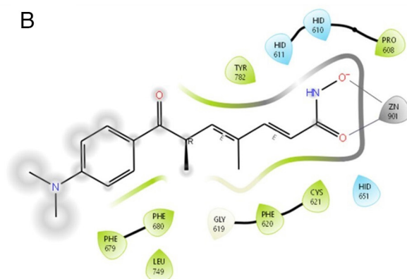
Figure S3. 2D representation of the interactions of (A) TSA co-crystallized and (B) TSA docked within the histone deacetylase 6 active site for validation purposes. TSA, trichostatin A.
