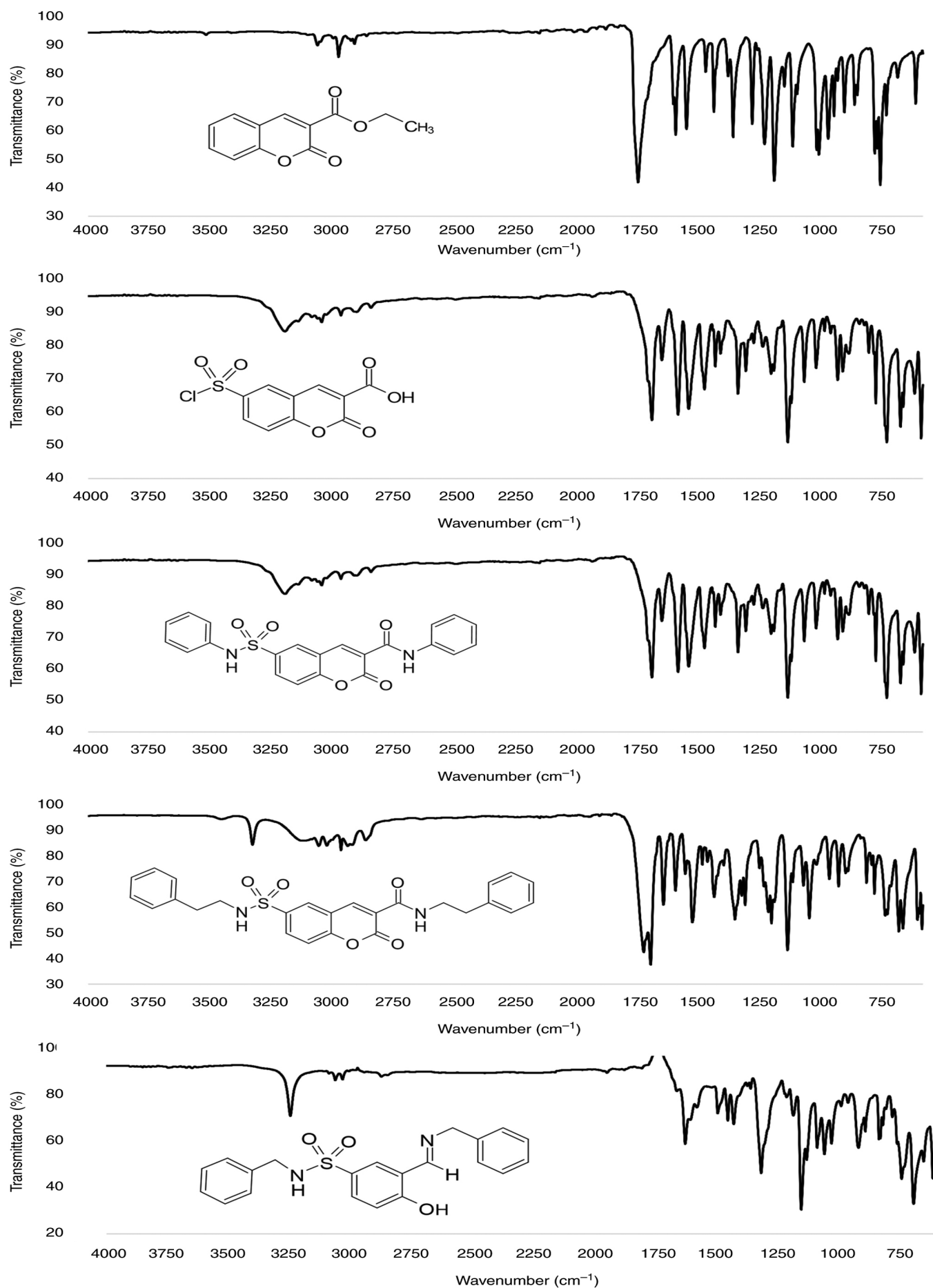
Figure S1. IR spectra ( \text{cm}^{-1} ) of compounds 2, 3, 4a, 4c and 5.
