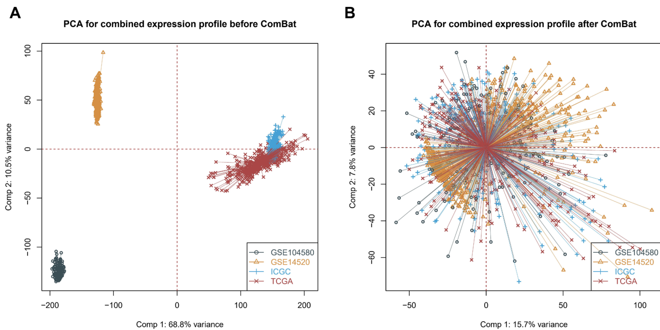
Figure S1. Comparison of data distribution after background correction and normalization using the sva R package. (A) PCA for combined expression profile before ComBat. (B) PCA for combined expression profile after ComBat.
