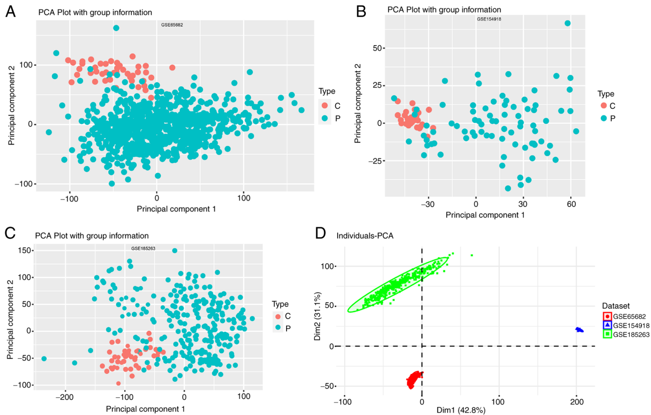
Figure S1. Heterogeneity between sepsis and normal samples across different datasets. PCA results demonstrated differences between sepsis and healthy samples in (A) GSE65682, (B) GSE154918 and (C) GSE185263 datasets. (D) PCA showed heterogeneity among the GSE65682, GSE154918 and GSE185263 datasets. PCA, principal component analysis; C, control; P, patient with sepsis; Dim, Dimension.
